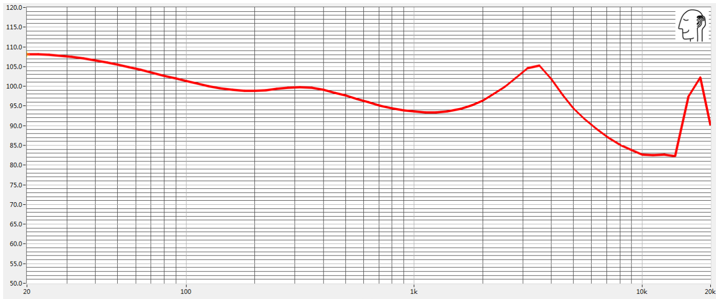
Frequency Response
