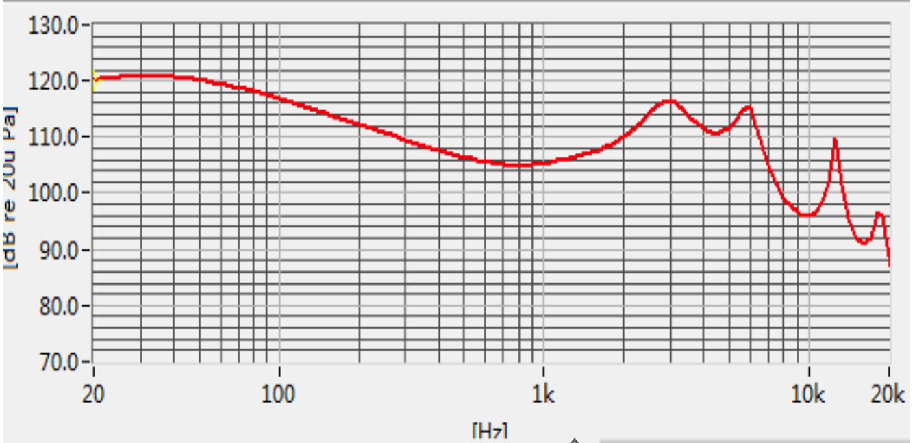
Frequency Response
