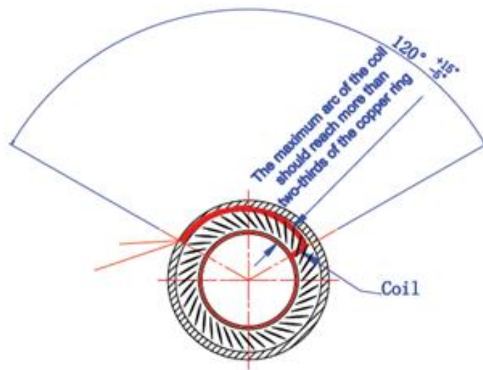
Diaphragm and Voice coil Ass'm
