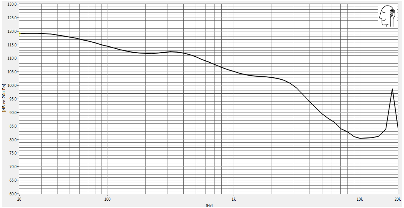
Frequency Response
